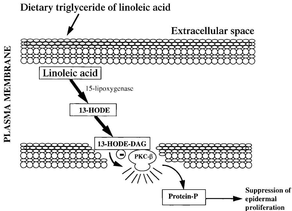
FIGURE 3. A speculative scenario showing how dietary linoleic acid could suppress skin hyperproliferation via cutaneous generation of putative 13-hydroxyoctadecadienoic acid (13-HODE)-substituted diacylglycerol (13-HODE-DAG). PKC- \beta , protein kinase C- \beta ; protein-P, phosphorylated protein.
