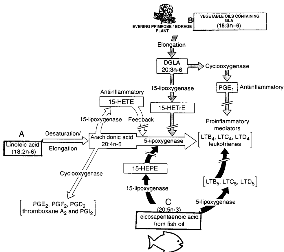
FIGURE 5. A speculative scenario of the possible attenuating effects of the constituent polyunsaturated fatty acids and metabolites from vegetable and fish oils on the generation of proinflammatory leukotrienes from arachidonic acid (AA). The A pathway illustrates the metabolic transformations from dietary intake of safflower oil, which is rich in linoleic acid (LA). It shows the in vivo desaturation and elongation of LA to AA followed by 5-lipoxygenation of AA to proinflammatory leukotrienes (LTs) (particularly LTB 4 ) by polymorphonuclear cells. AA is also metabolized by 15-lipoxygenase to 15-hydroxyeicosatetraenoic acid (15-HETE), which exerts antiinflammatory activity in the skin (28). The B pathway illustrates the epidermal elongation of dietary \gamma -linolenic acid (GLA), a constituent of evening primrose and borage oils, to dihomogamma-linolenic acid (DGLA), followed by 15-lipoxygenation of DGLA to 15-hydroxyeicosatrienoic acid (15-HETE) and cyclooxygenation to prostaglandin E 1 (PGE 1 ). The C pathway illustrates the 15-lipoxygenation of dietary eicosapentaenoic acid to 15-hydroxyeicosapentaenoic acid (15-HEPE) and the 5-lipoxygenation to LTB 5 .
