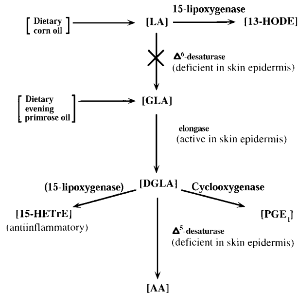
FIGURE 1. Metabolism of dietary linoleic acid (LA) and \gamma -linolenic acid (GLA) in skin epidermis. 13-HODE, 13-hydroxyoctadecadienoic acid; DGLA, dihomo- \gamma -linolenic acid; 15-HETrE, 15-hydroxyeicosatrienoic acid; PGE 1 , prostaglandin E 1 ; AA, arachidonic acid.
