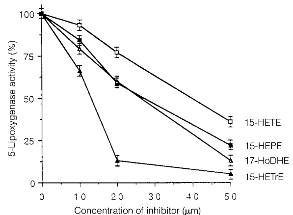
FIGURE 4. Inhibition of RBL-1 leukemia cells' 5-lipoxygenase-catalyzed transformation of arachidonic acid to leukotriene B 4 by the monohydroxy fatty acids 15-hydroxyeicosatetraenoic acid (15-HETE), 15-hydroxyeicosapentaenoic acid (15-HEPE), 17-hydroxydocosahexaenoic acid, (17-HoDHE), and 15-hydroxyeicosatrienoic acid (15-HETrE). The inhibitory effects of these monohydroxy fatty acids were ascertained by incubation with RBL-1 cell homogenates. Each point represents the mean \pm SEM of triplicate determinations from 3 separate experiments. From reference 22.
